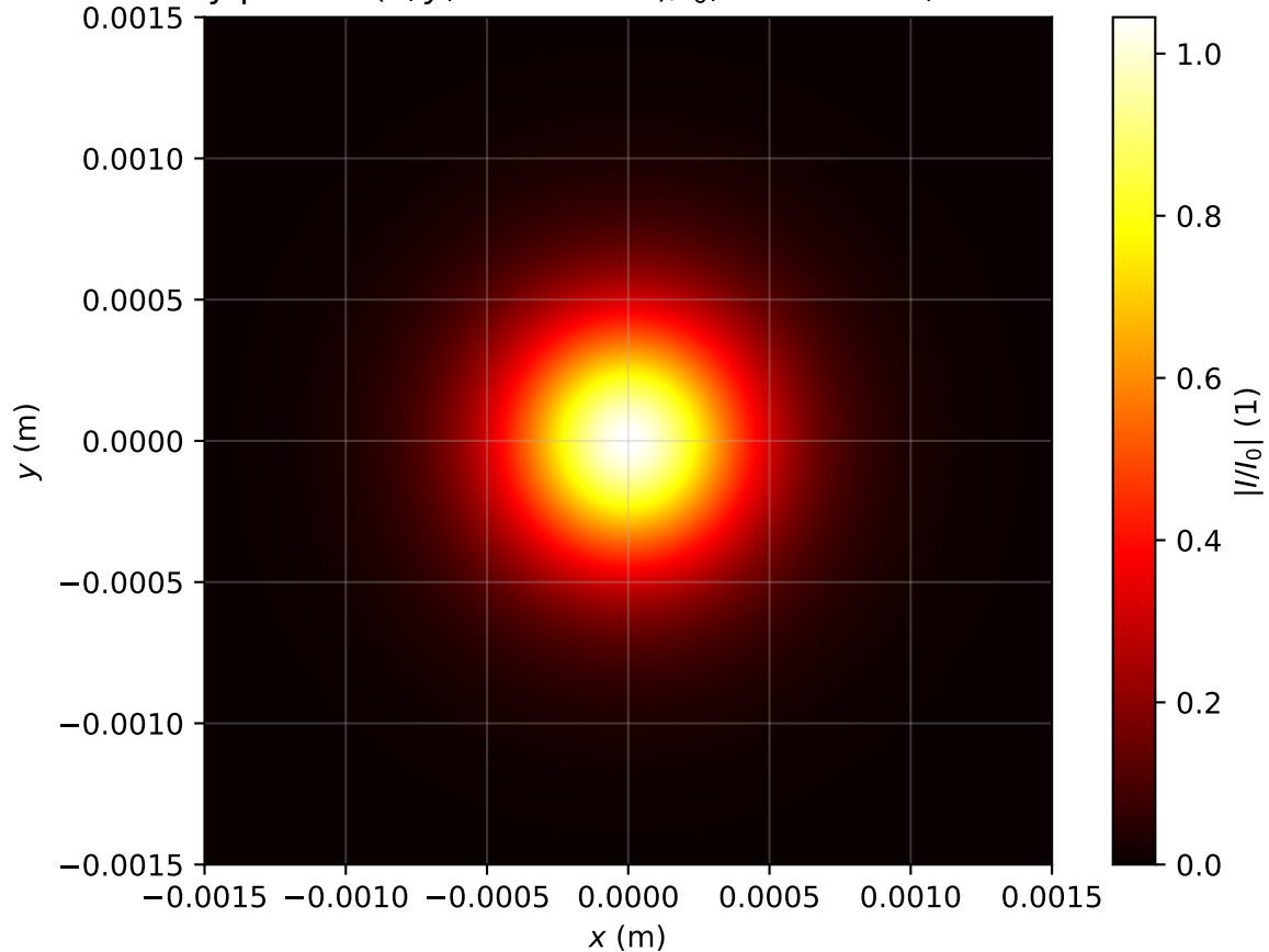
Intensity profile I(x, y, z = 1.592m)/I_0 , Pin=0.6Pcr, artificial time
